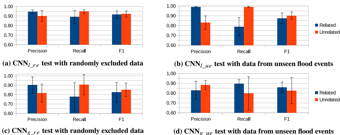
Figure 2. Averaged results of local and global models tested with randomly excluded and new flood event data
