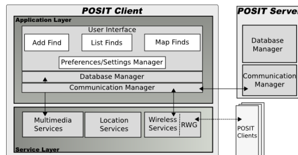
Figure 1. POSIT Architecture
