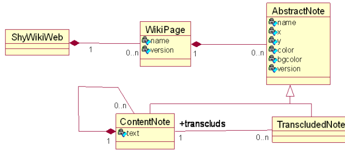
Figure 6. ShyWiki Hypertext Model
