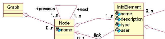
Figure 5. Knowledge Graph Model (partial)
