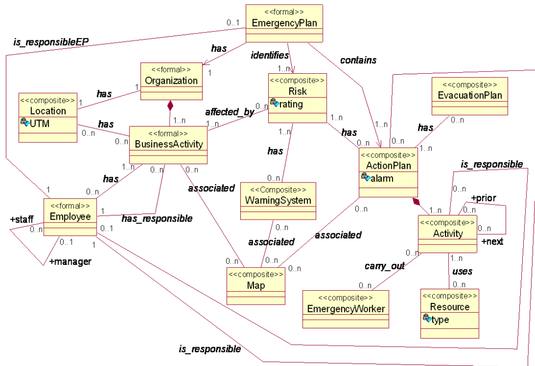
Figure 4. Emergency Response Plan Model based on the NBA.
