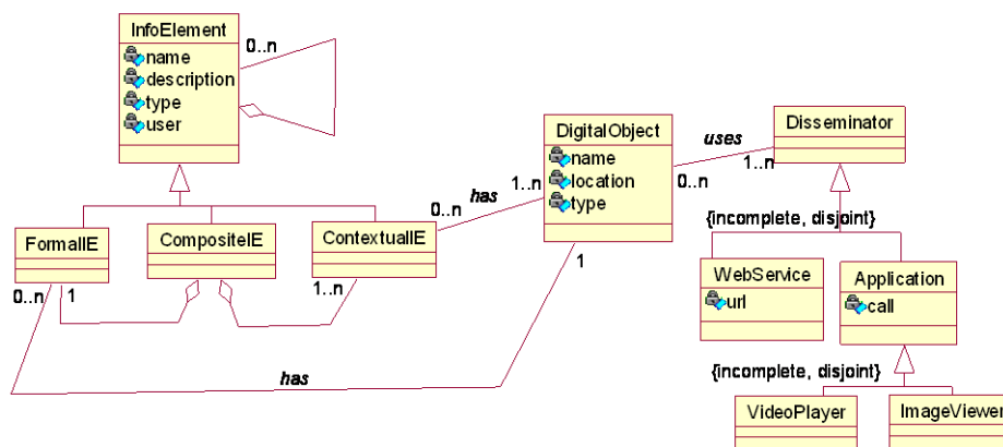
Figure 3. Knowledge Model including Composite Knowledge
