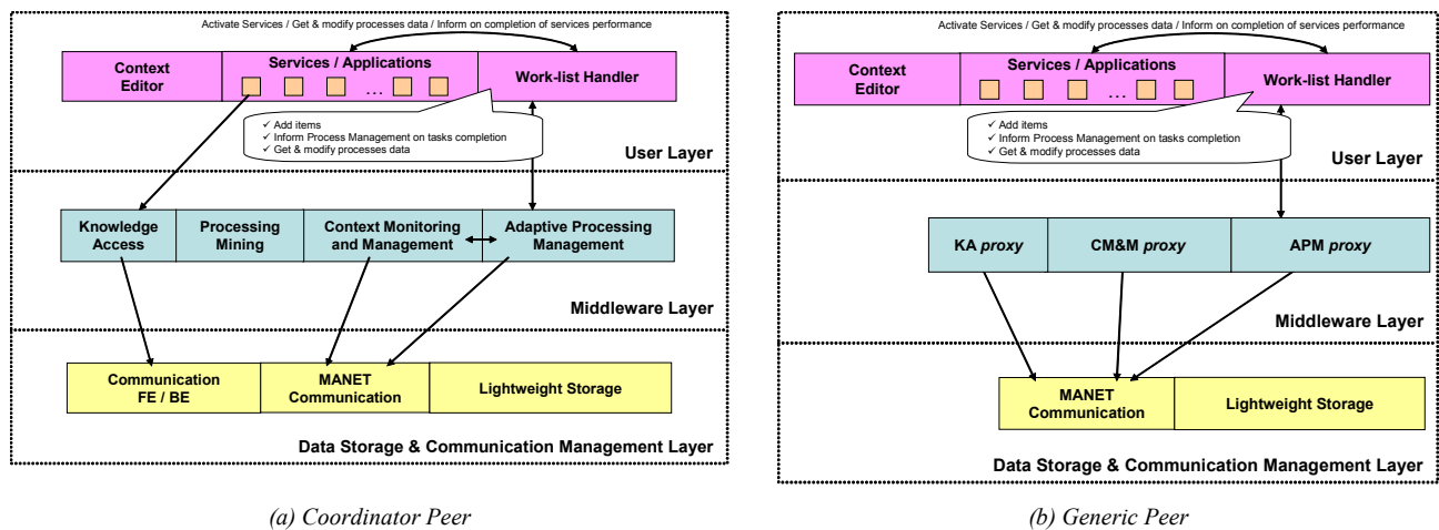
Figure 4. Front-end Architecture
