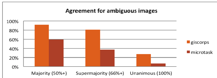
Figure 2: Tough-to-classify images (count = 720) rated by experts. They received pretty consistent ratings by the experts but note that these images were chosen *because* non-experts had substantial disagreement.
